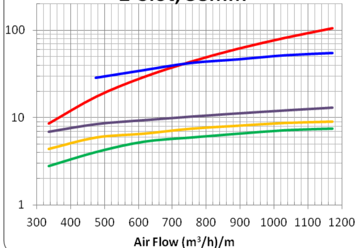
2-Slot, 38mm
