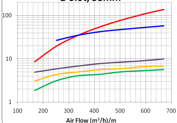
1-Slot, 38mm
