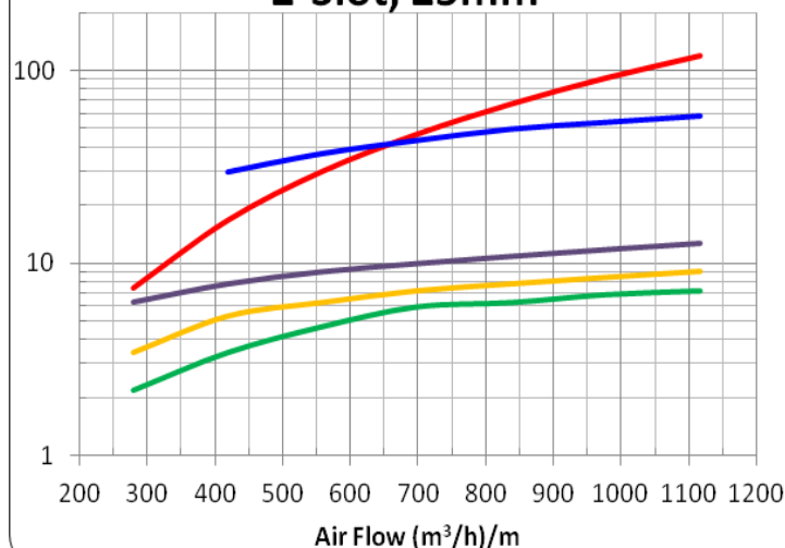
2-Slot, 25mm
